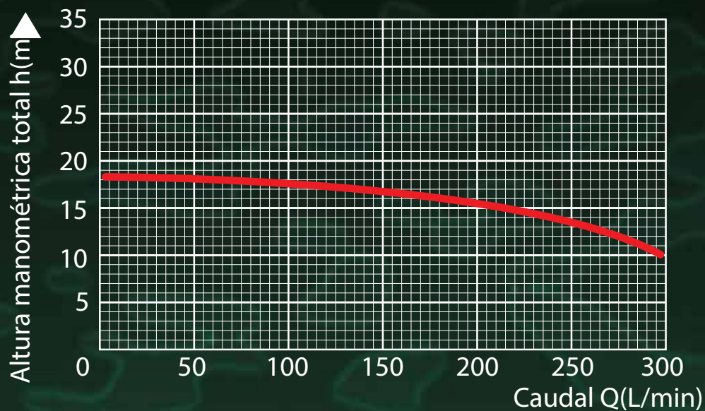
PERFORMANCE AT n=2850 l/min
